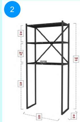
13-03-03 METAL BATHROOM ORGANIZER
